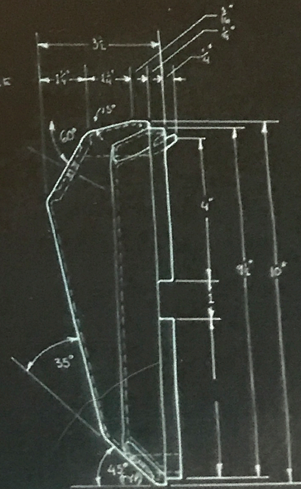
SIDE VIEW
